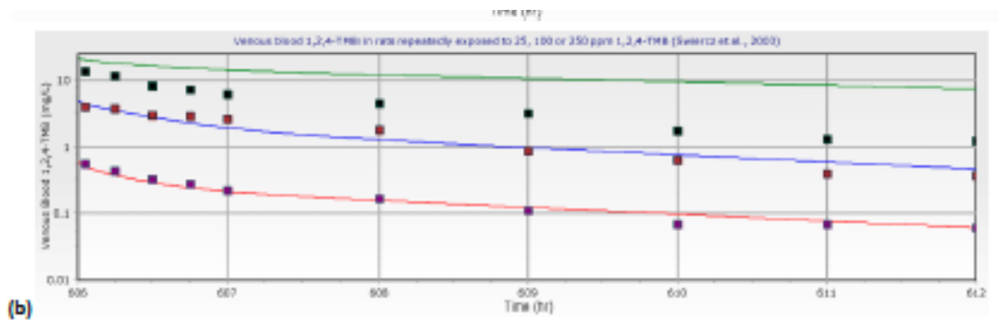
Swiercz et al. (2003) in rats repeatedly exposed to 1,2,4-TMB: (a) before and (b) after numerical optimization. See Legend in Figures B-7 and B-8.
